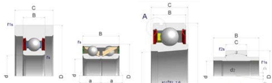
*5 - Special ball bearing covered by metal shields and with extended outer ring, with radial clearance Gr 0,005 to 0,020 mm.
