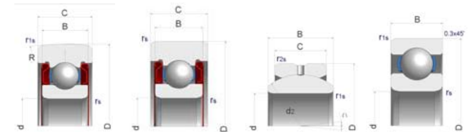
*1 - When using the bearing as relieving pulley the values for load rating Cr, Cor and limiting rotation speed are decreased on 2/3 of the values specified in the table.
