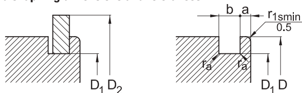
Snap ring groove
