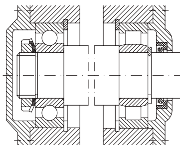
locating bearing a) non-locating bearing
