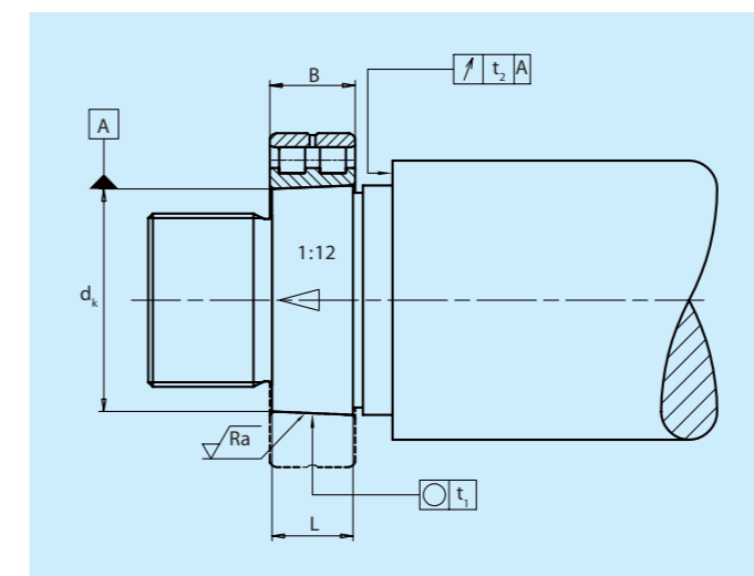
Fig. 17.2. Machining of tapered shafts
