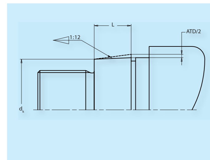
Fig. 17.3. Machining of tapered shafts (detail)
