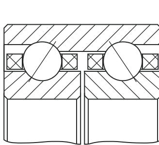
M-Type SuperDuplex™ Back-to-Back
