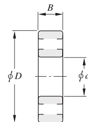
Cylindrical bore
