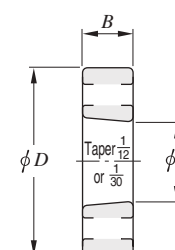
Tapered bore
