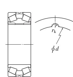
Bore key way
