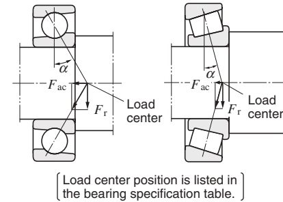
Fig. 1-1 Axial component force
