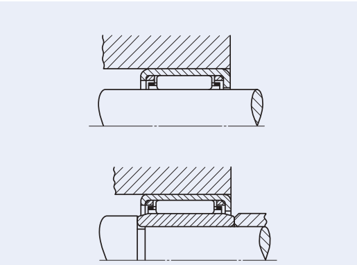
Fig.2 Mounting examples
