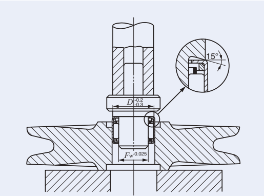
Fig.1 Example of mounting tool
