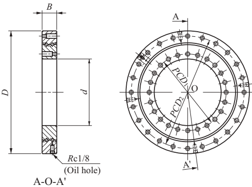
Fig. 5 Manufacturing example
