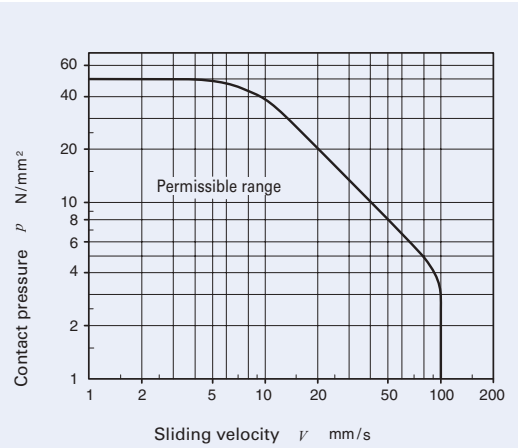
Fig. 2 pV diagram of lubrication type PILLOBALLS
