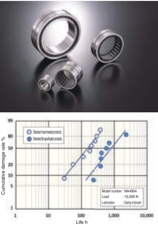
Fig. 1 Life Test Result Remark This table shows the result of life testing under load conditions at 50% of the basic dynamic rating. The Extended Life Specification with special heat treatment lasted 5 times longer or more in L10 life compared to the standard heat-treated products.
